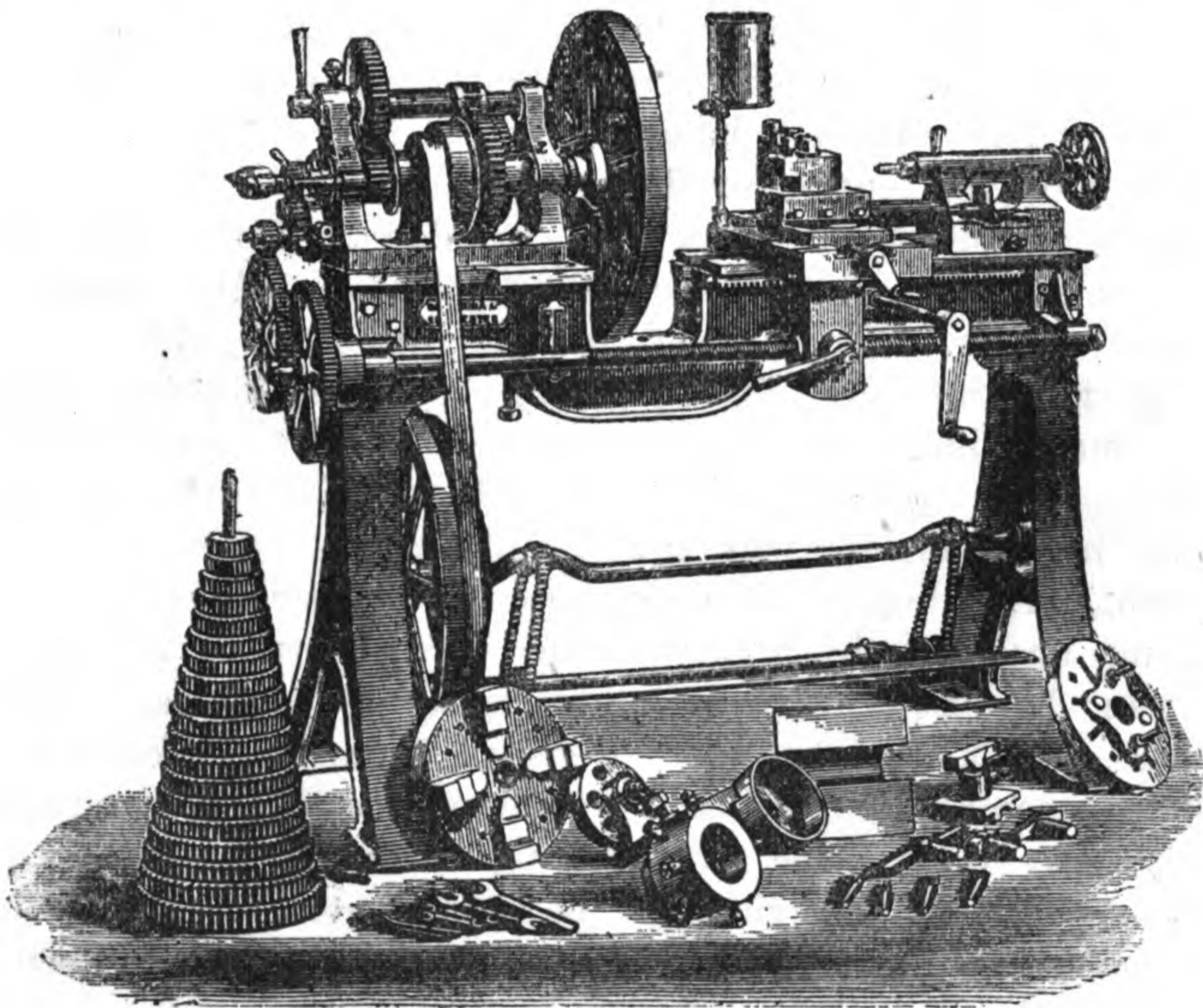
FIG. 21.—TREBLE-GEARED LATHE.
