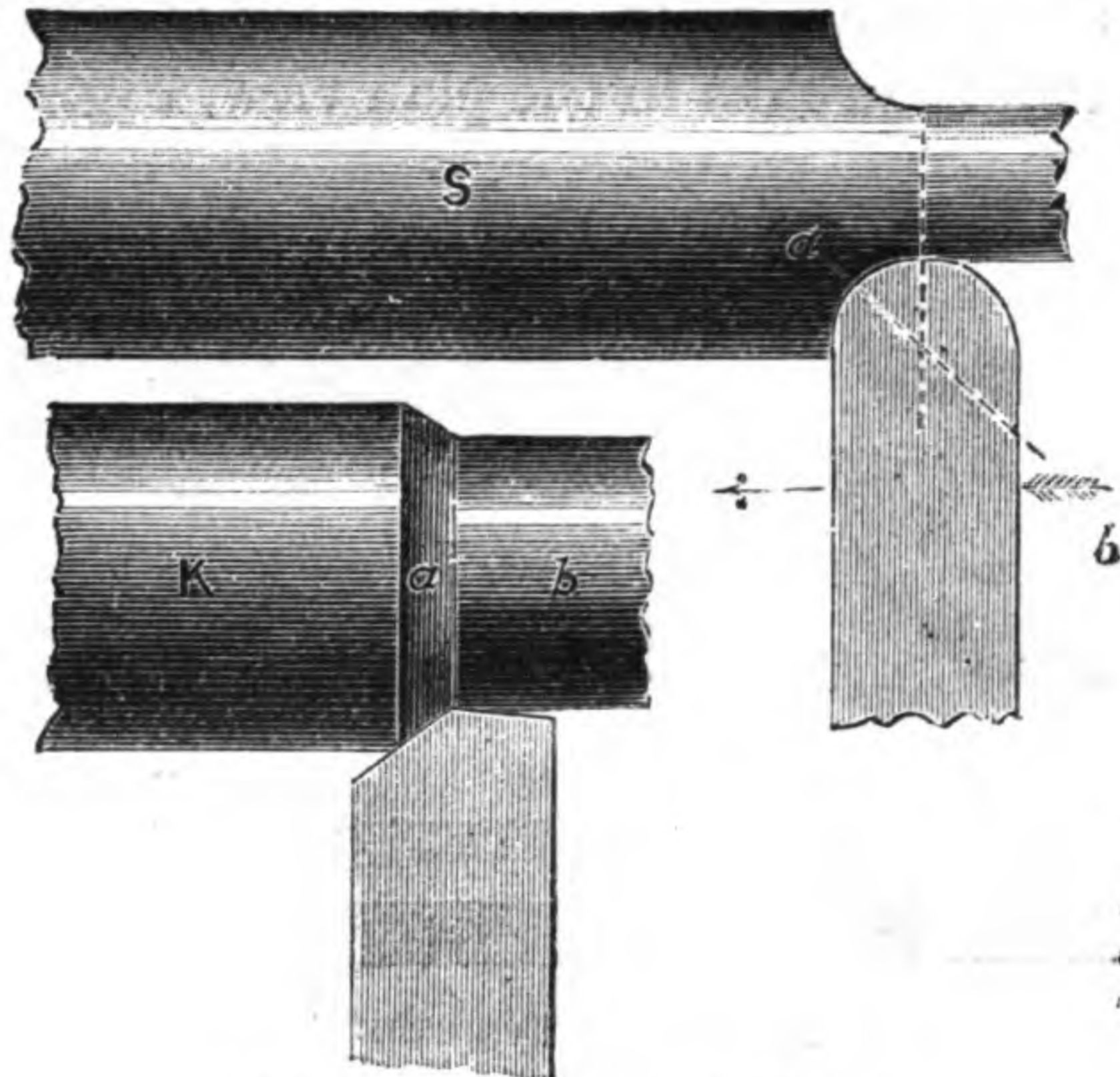
FIG 12.—SLIDE-REST WORK.
