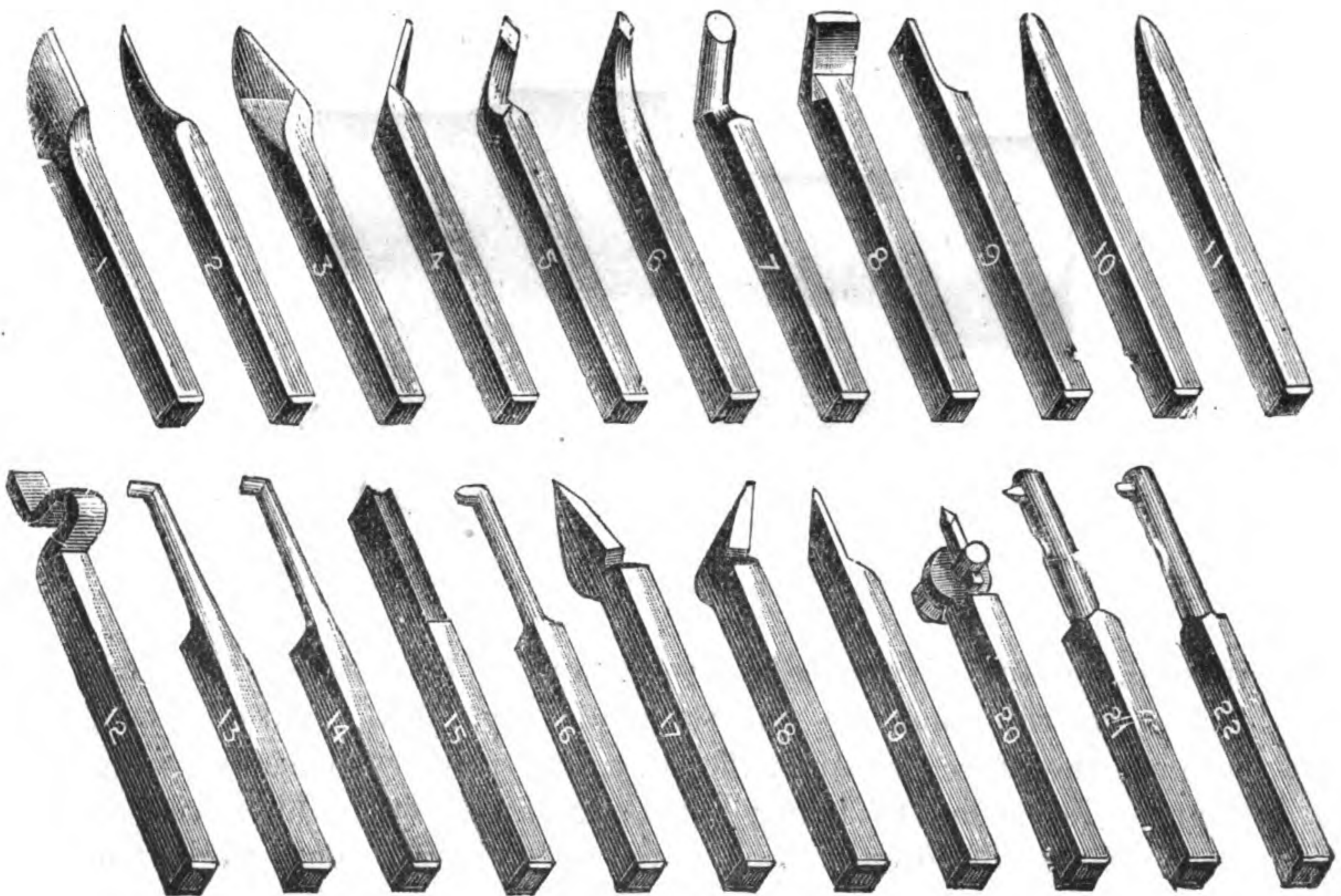
FIG. 15.—VARIOUS SLIDE-REST TOOLS.
