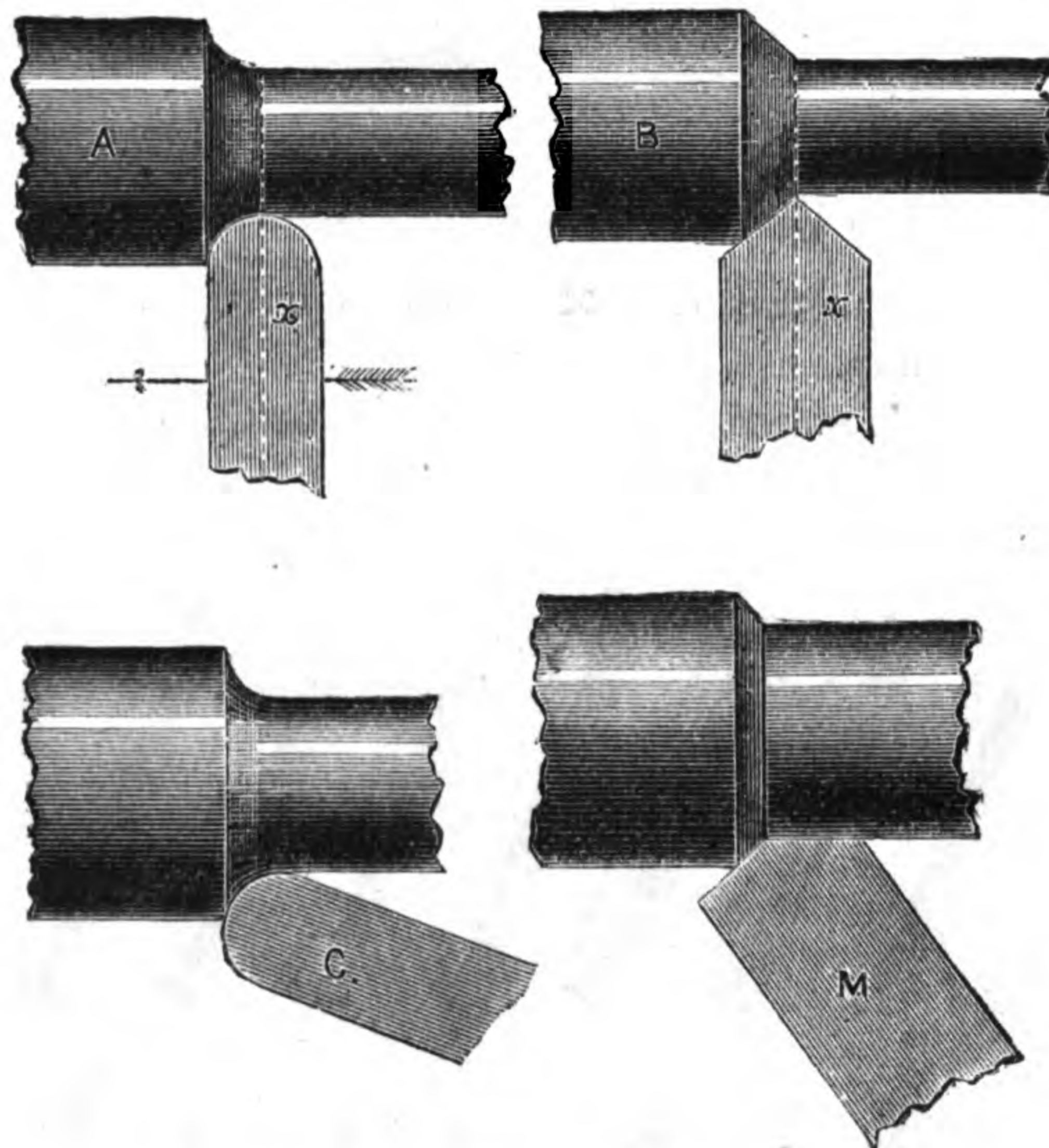
FIG. 13.—PRINCIPLE OF DOUBLE EDGES.
