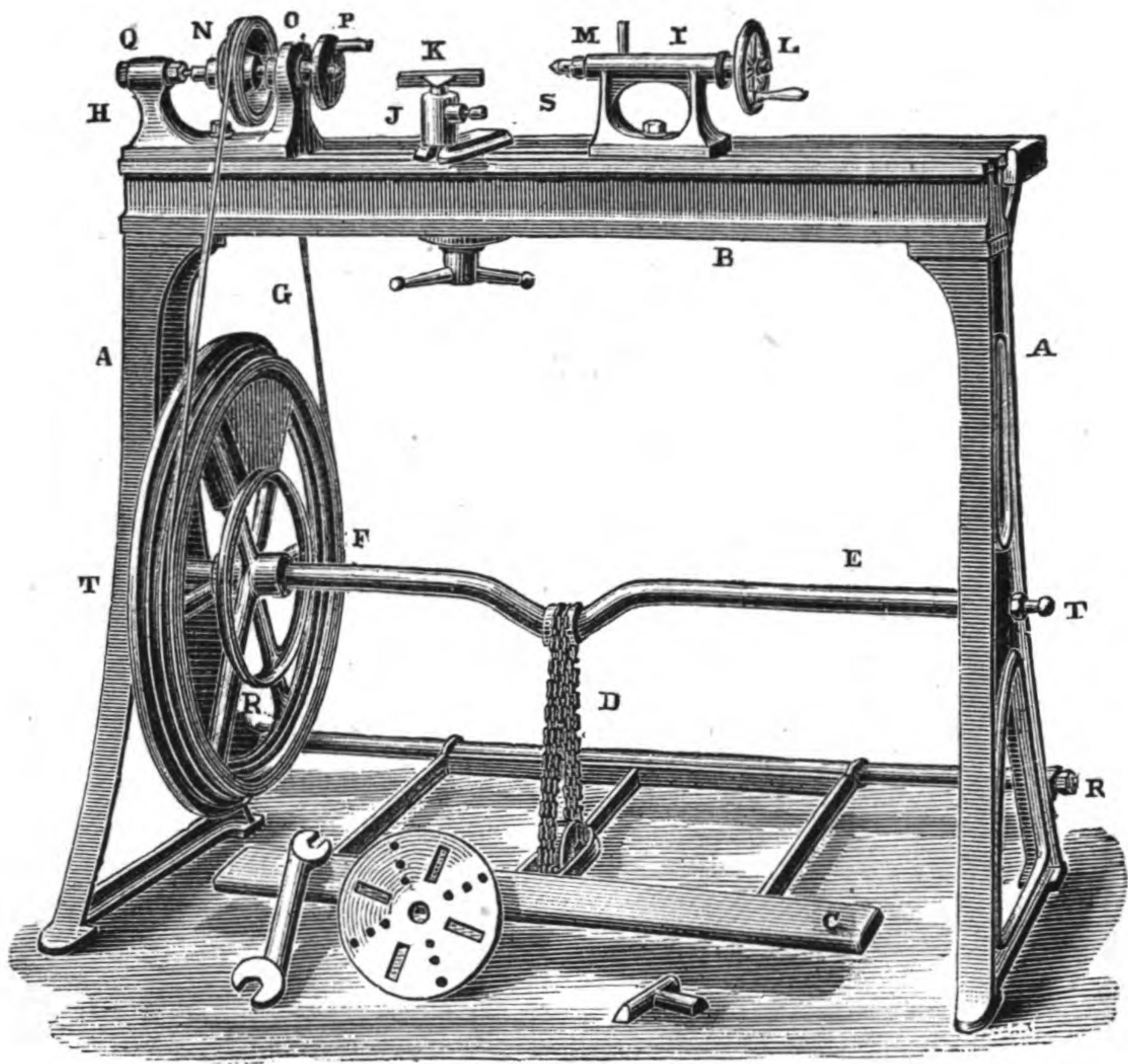
PLATE I.—PLAIN FOOT LATHE.
