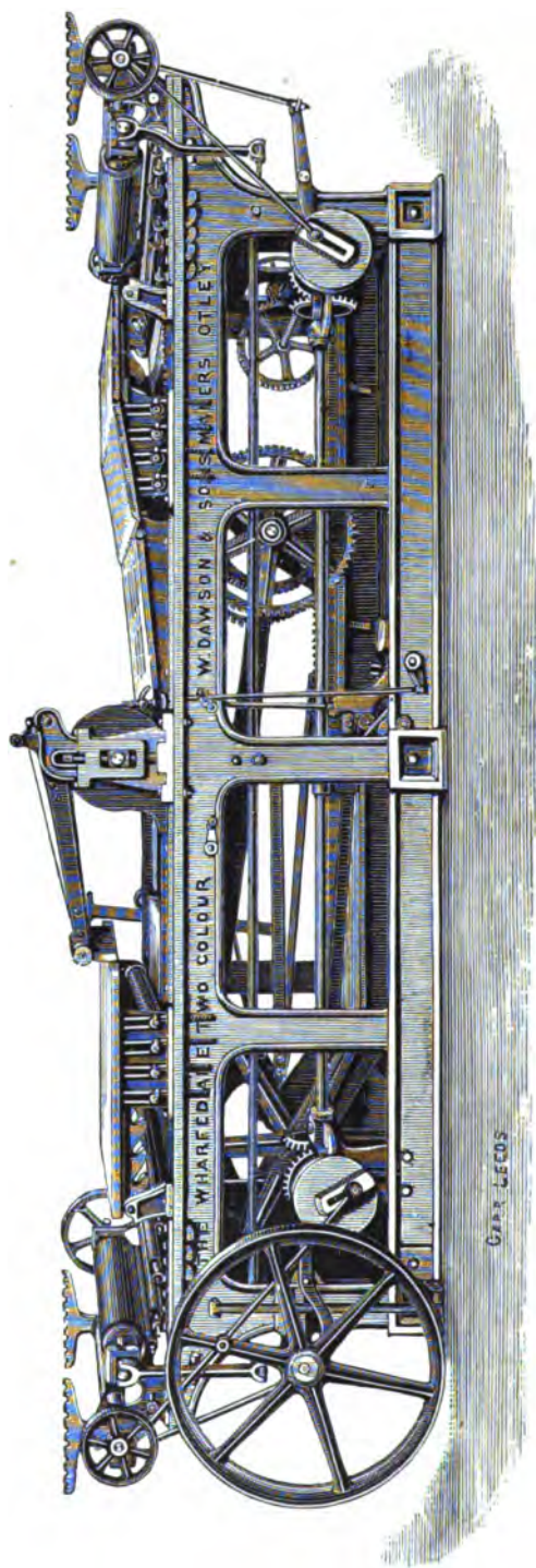
FIG. 29.—TWO-COLOUR MACHINE, WITH TAKING-OFF APPARATUS.
