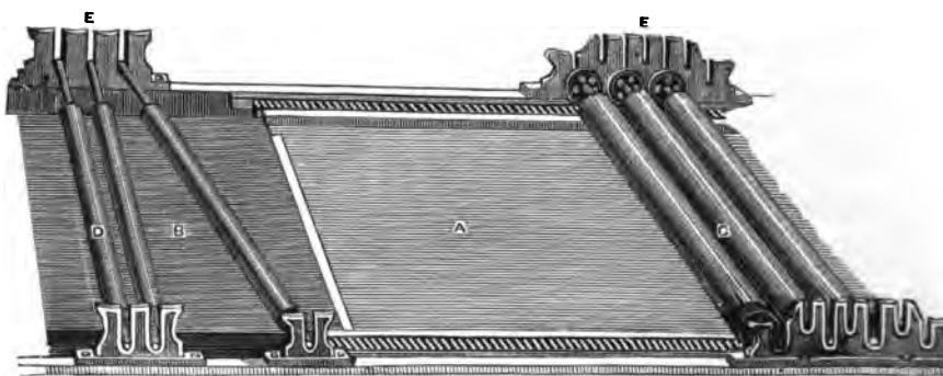
Fig. 17.—Coffin and Inking Slab, showing Arrangement of Rollers. A Coffin; B Inking slab; C Inker; D Waver; E E Roller forks.
