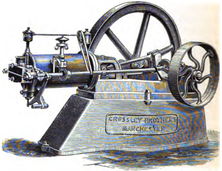
Fig. 136.—The Otto Gas Engine.
