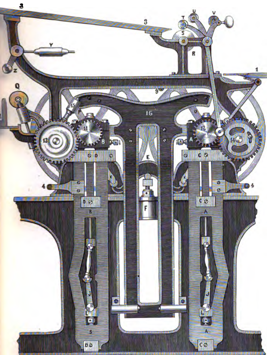
Fig. 70.—Showing Motions on the Near-side of Machine.
