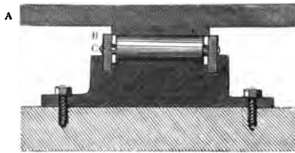
Fig. 13.—Section showing Table, Table-bar, and Runner.
