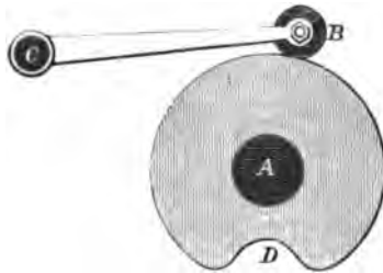
Fig. 46.—The Drop-bar Motion.
