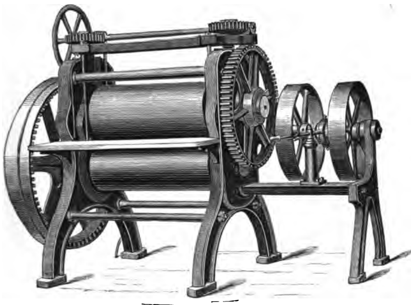
Fig. 107.--Rolling Machine with clutch Motion.
