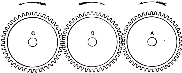
Fig. 9.—Reversing Motion.
