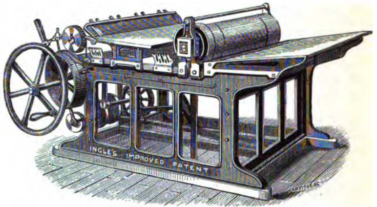
Fig. 14.—Ingle's Machine, showing Rocking-Lever Motion.
