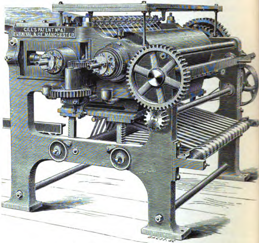
Fig. 121.—The Gill Hot-rolling Machine.
