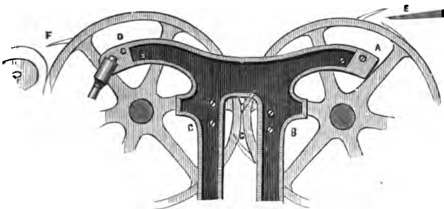
Fig. 68.—Folding Frame for opening and shutting Grippers.
