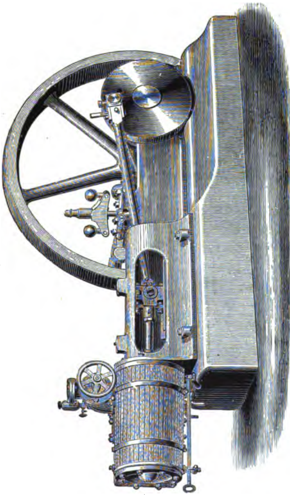
FIG. 135.—HORIZONTAL ENGINE.
