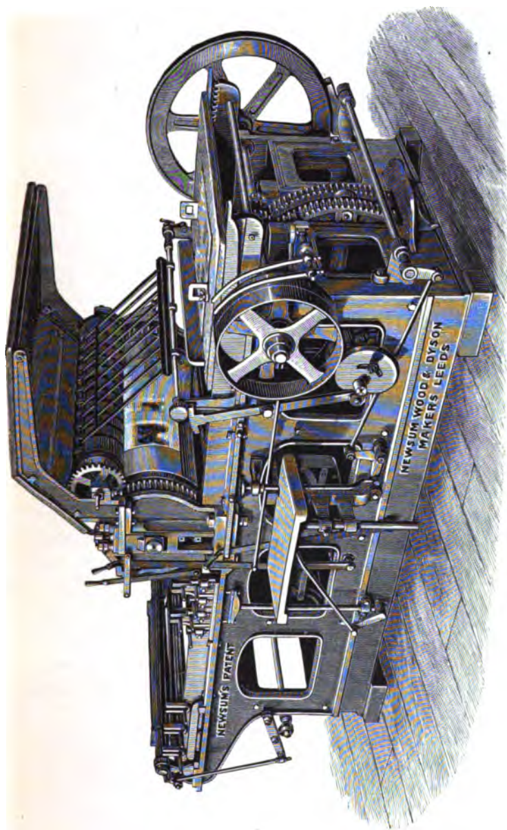
FIG. 24.—NEWSUM'S ANGLO-AMERICAN MACHINE.
