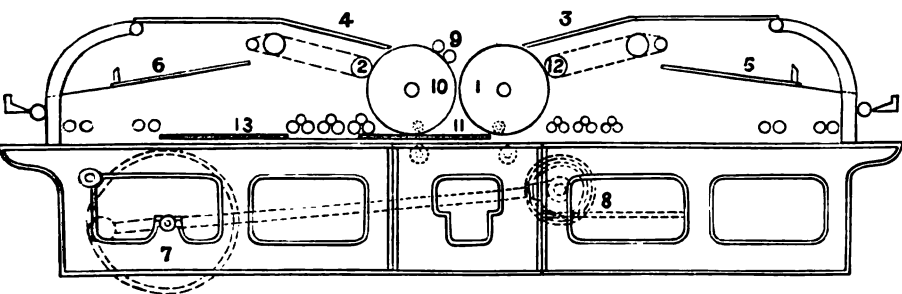
Fig. 52.—Newsum's Perfecting Machine.
