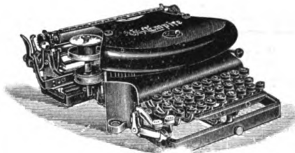
No. 1 MODEL The only portable and standard. Ordinary model weighs 16½ lbs. (7.5 kilos) Travellers " 10½ " (4.8 " ) The strongest and most reliable portable typewriter
