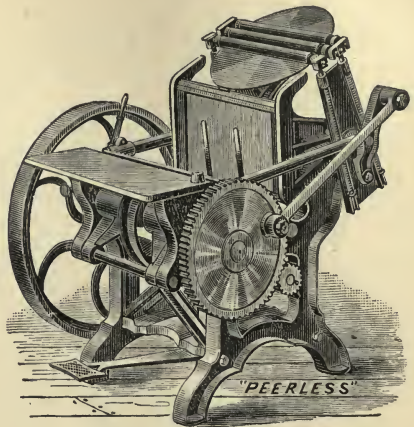
"Peerless" Job Press.
