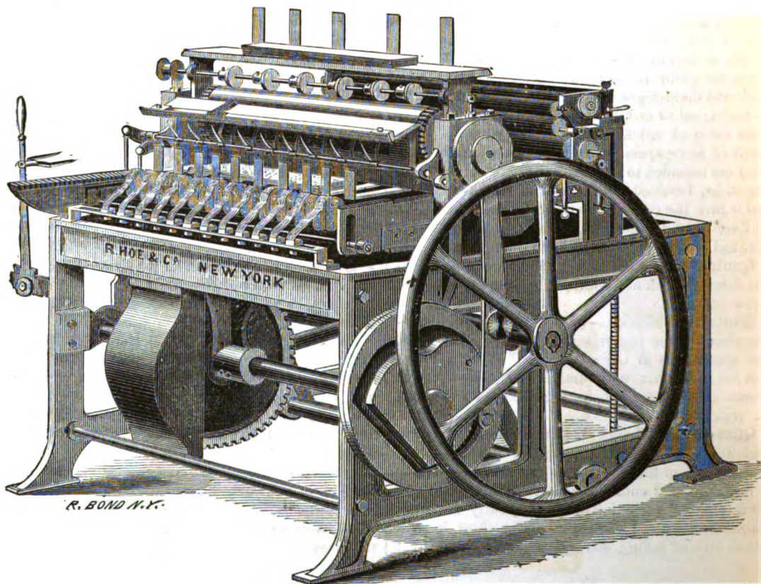
RAILWAY COUPON-TICKET PRINTING AND NUMBERING MACHINE.
