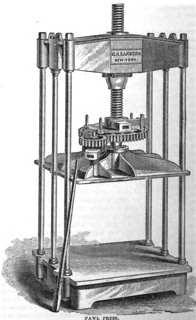
PAWL PRESS.
