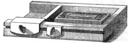
MAKE-UP GALLEY.
