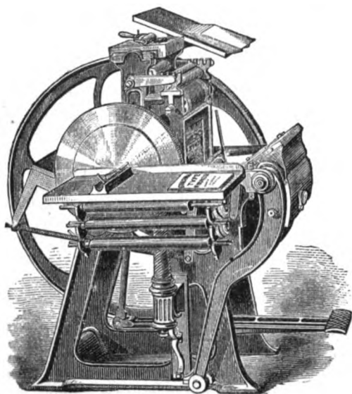
NONPAREIL PRESS.
