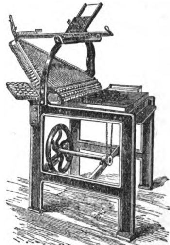
HATTERSLEY DISTRIBUTING MACHINE.
