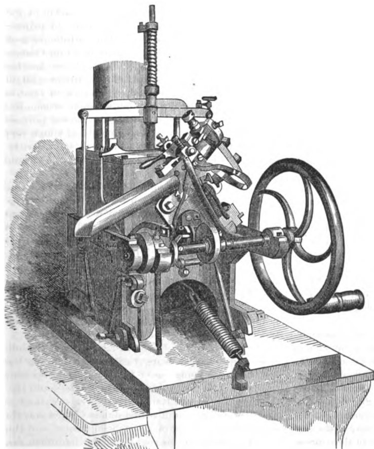
TYPE-CASTING MACHINE.
