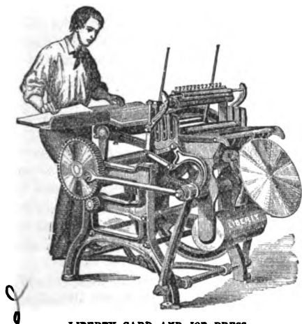
LIBERTY CARD AND JOB PRESS.
