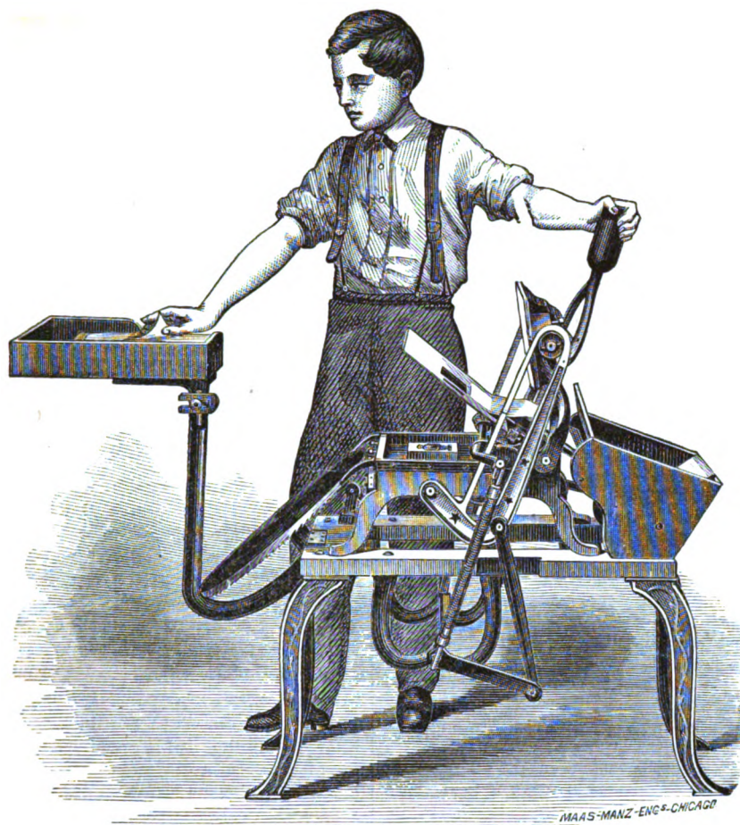
KELLOGG IMPROVED NEWBURY BLANK AND CARD PRESS.
