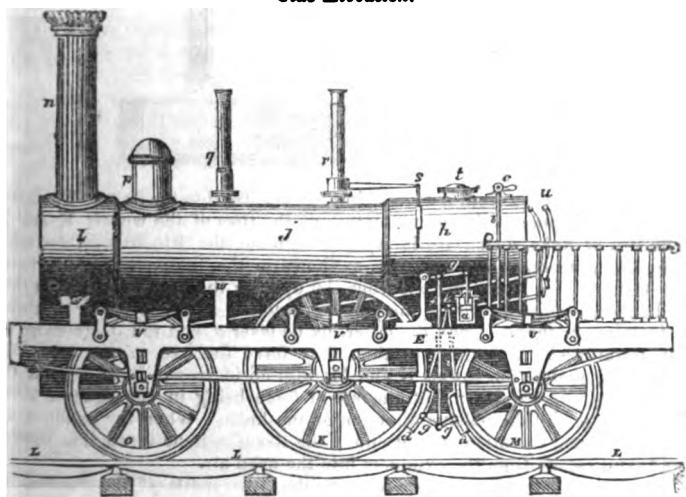
Side Elevation.
