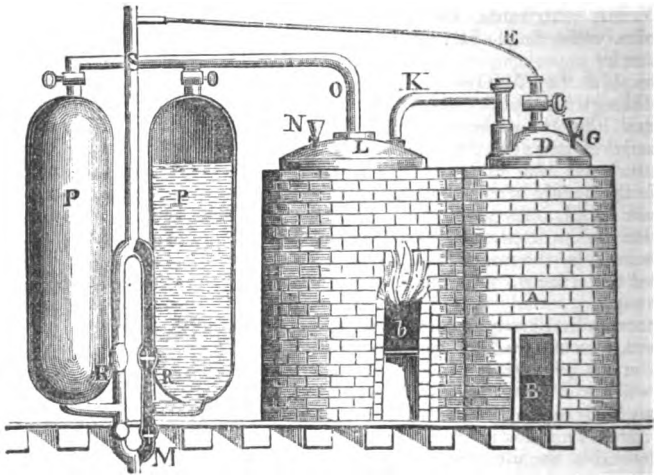
Savery's Engine, 1699.
