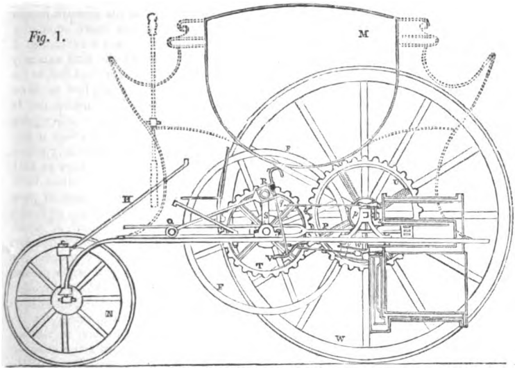
TREVITHICK AND VIVIAN'S STEAM CARRIAGE.—PATENT 1802.
