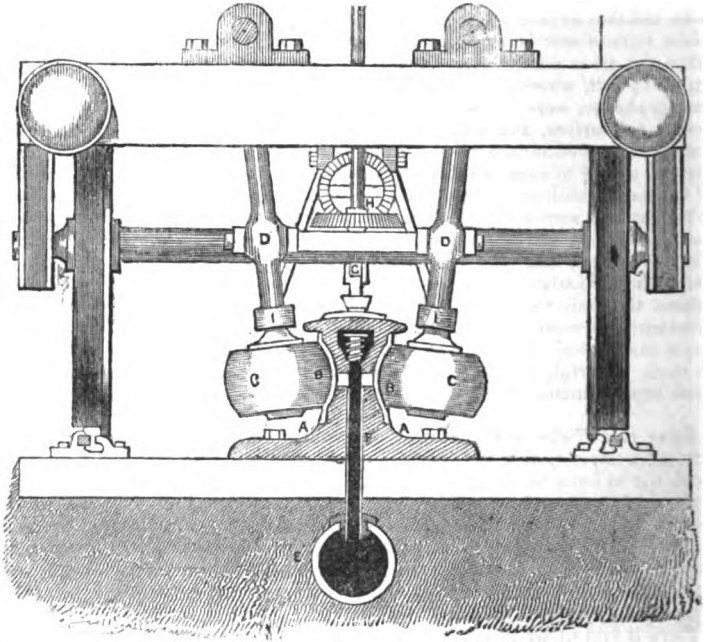
THE CUT REPRESENTS A TRANSVERSE SECTION OF THE APPARATUS.
