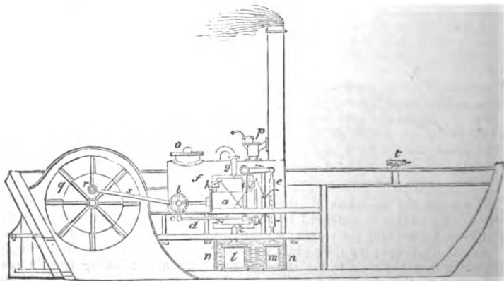
The cut above represents a partial section of the Charlotte Dundas , one of the vessels constructed by Mr. Symington for Lord Dundas, and which in the
