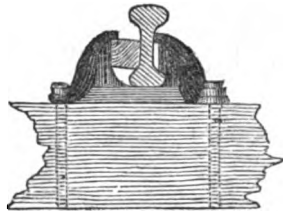
Elevation of Chair, showing the inclination of the Rail.
