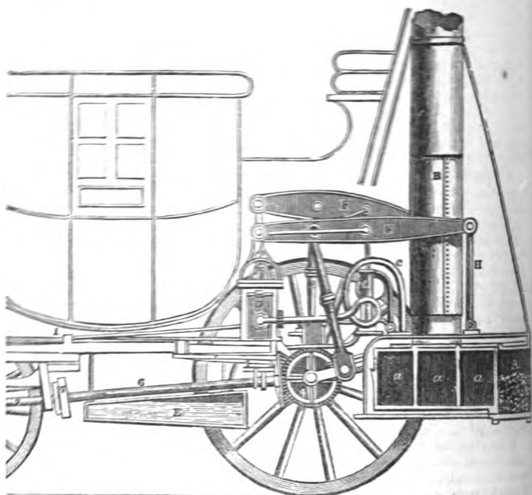
BURSTALL AND HILL'S STEAM CARRIAGE.—PATENT 1824.
