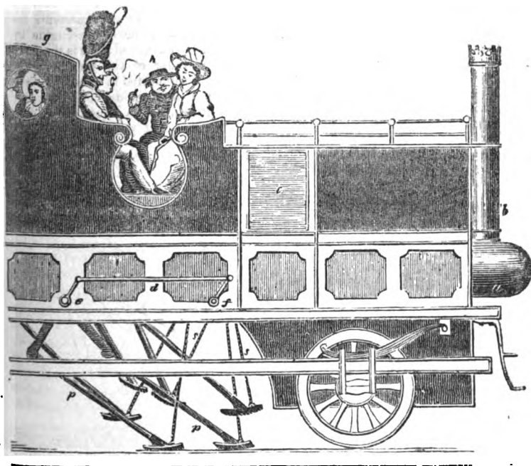
DAVID GORDON'S STEAM CARRIAGE.—PATENT 1824.
