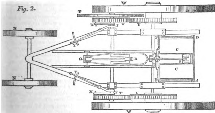
TREVITHICK AND VIVIAN'S STEAM CARRIAGE.—PATENT 1802.
