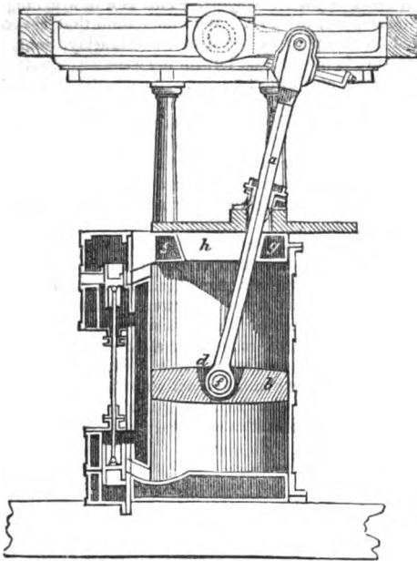
PARKYN'S ENGINE.
