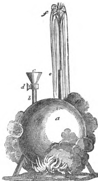
DE CAUS'S ENGINE, 1615.
