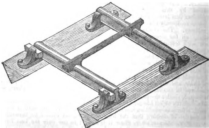
Rails, Chairs, and Sleepers, with the clamp gauge fixed.
