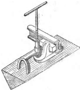
Guide Tube, and Spiral Auger, in use.
