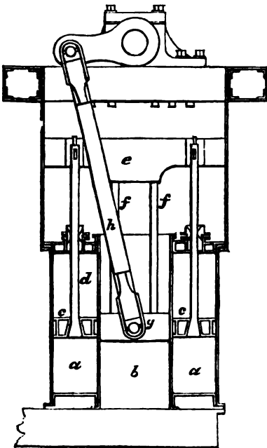
MAUDSLAY'S ANNULAR CYLINDER ENGINE.
