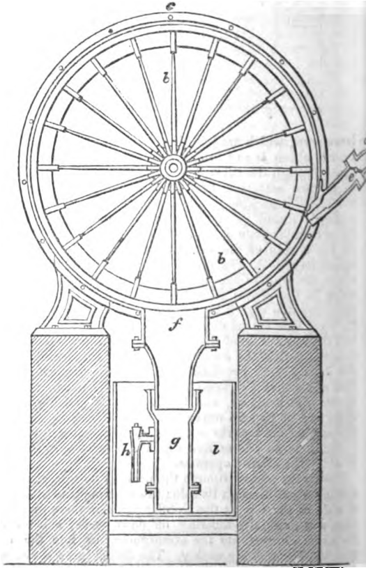
CORDER AND LOCKE'S ROTATORY ENGINE.
