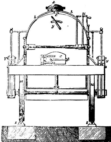
End Elevation.
