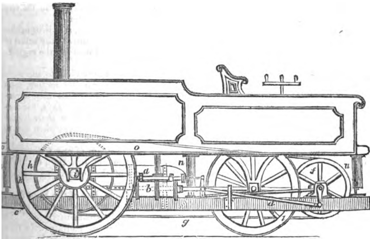
NAPIER'S STEAM CARRIAGE—PATENT 1831.
