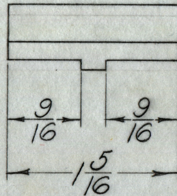
Straddle Mill
