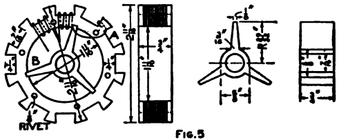
Fig. 6 Armature-Ring Core, Its Hub and the Construction of the Commutator and Its Insulation
