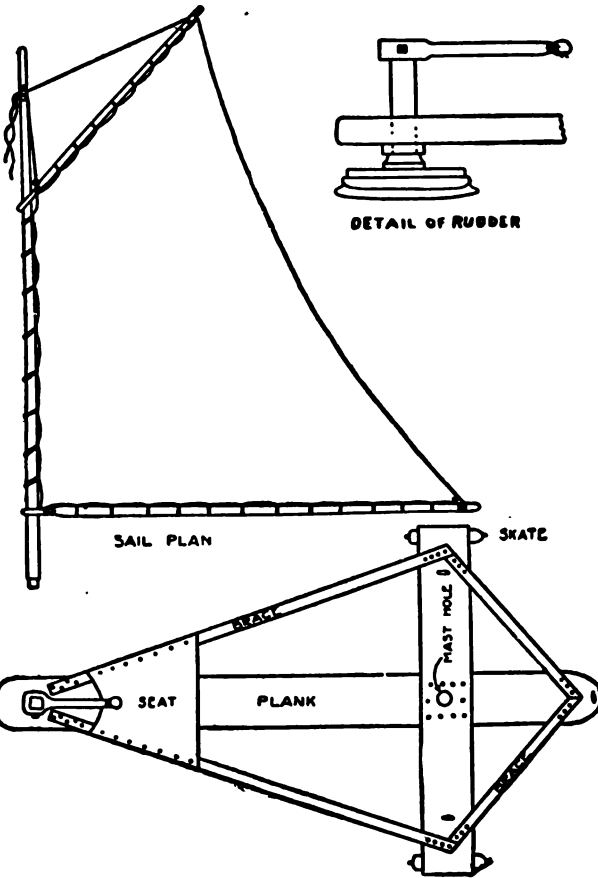
Plan of Ice Boat, Sail and Rudder
