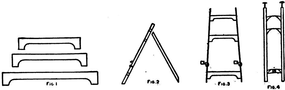
Details of Easel Construction
