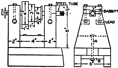
FIG 6 Headstock Details
