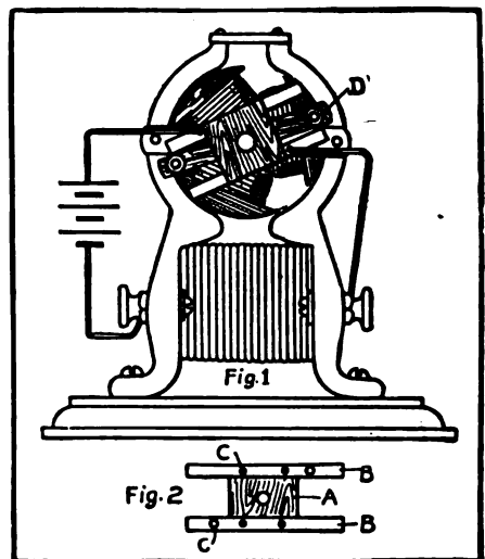
Direct-Connected Reverse
