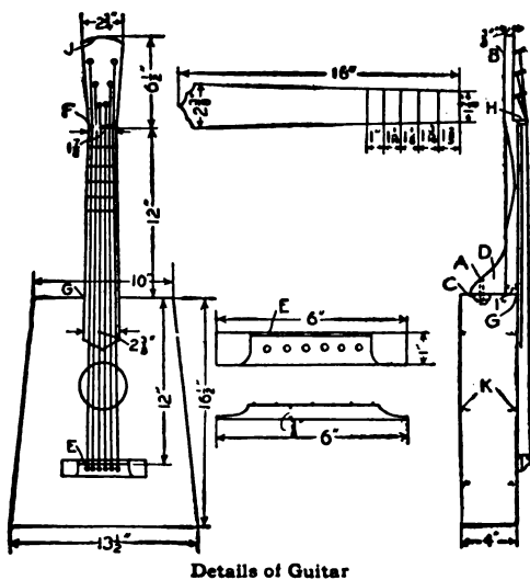
Details of Guitar
