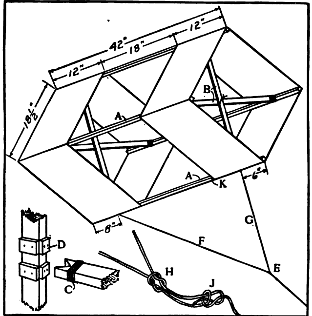
Detail of Box Kite
