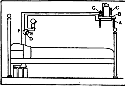
Handy Electric Alarm
