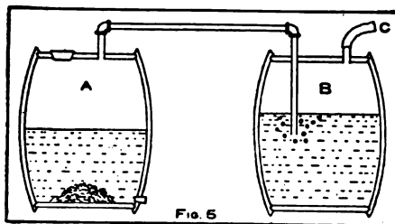
The Hydrogen Generator
