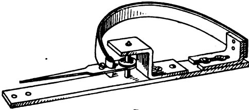
FIG. 13 Assembled Thermostat
