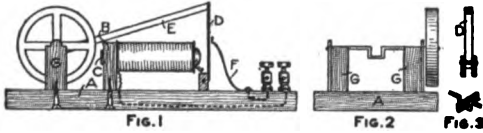
Shaft Turned by Magnetism
