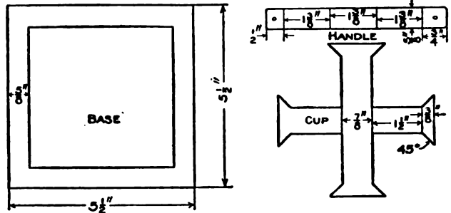
Details of Candle Holder
