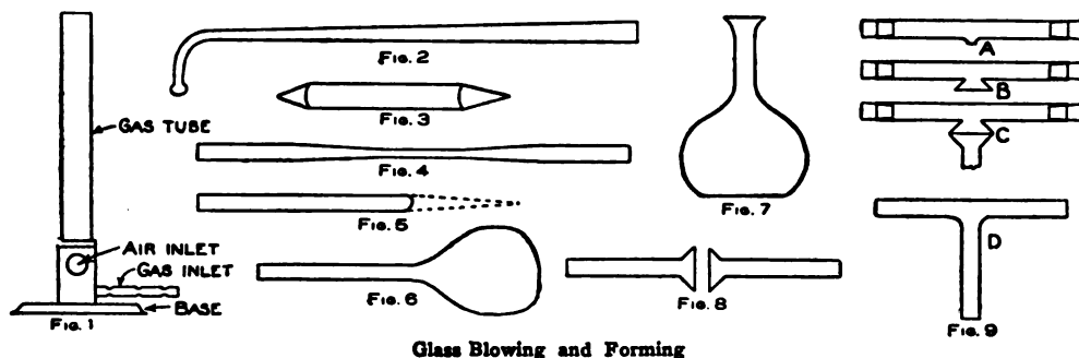
Glass Blowing and Forming
