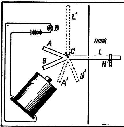
Lock Operated by a Magnet
