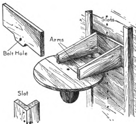
Adjustable Platform
