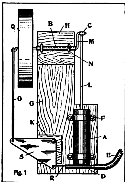
Toy Steam Engine Assembled
