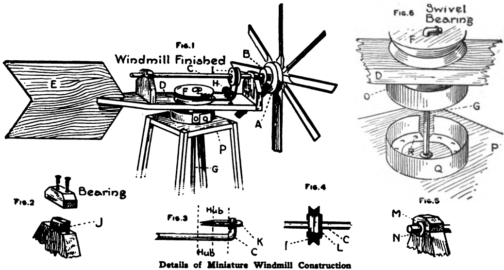
Details of Miniature Windmill Construction
