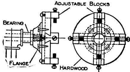
Fig. 4-Chuck
