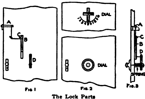
The Lock Parts
