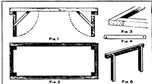
Details of Canvas Cot Construction
