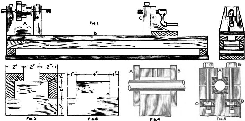
Assembled Lathe Bed and Bearing Details
