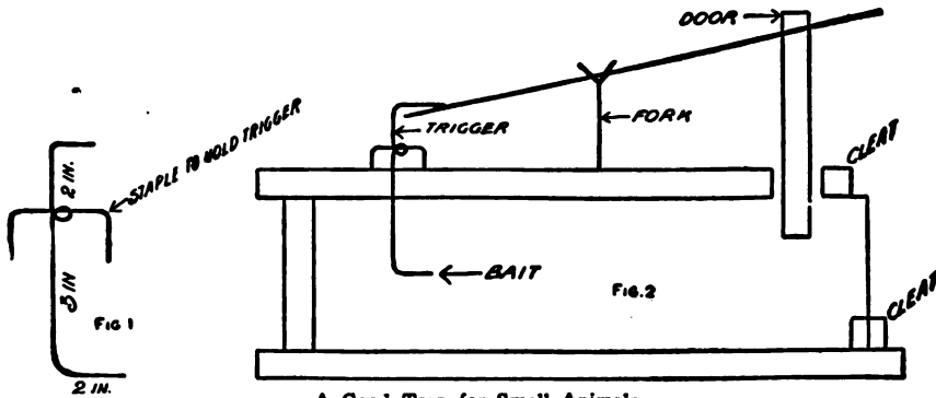
A Good Trap for Small Animals
