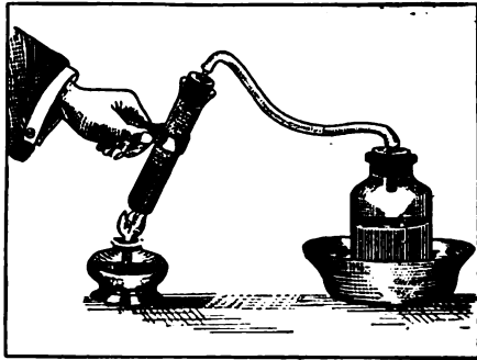
Distilling Water
