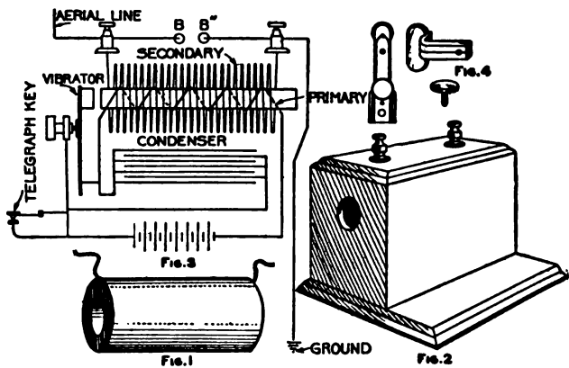
Jump-Spark Coil
