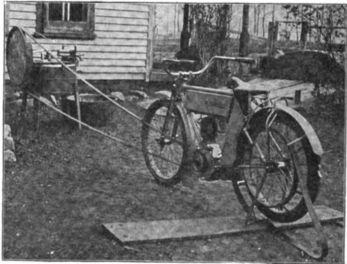
Machine Belted to the Motorcycle
