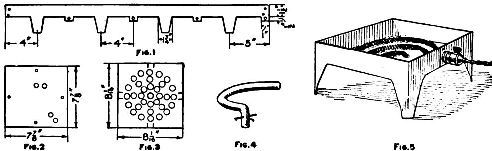
Pattern for Parts of the Electric Stove
