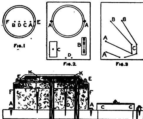
Fig. 4 Details of Electric Stove
