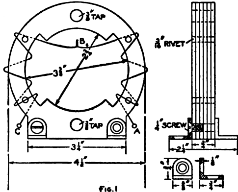
FIG. 1 The Field-Coil Core is Built Up of Laminated Wrought Iron Riveted Together
