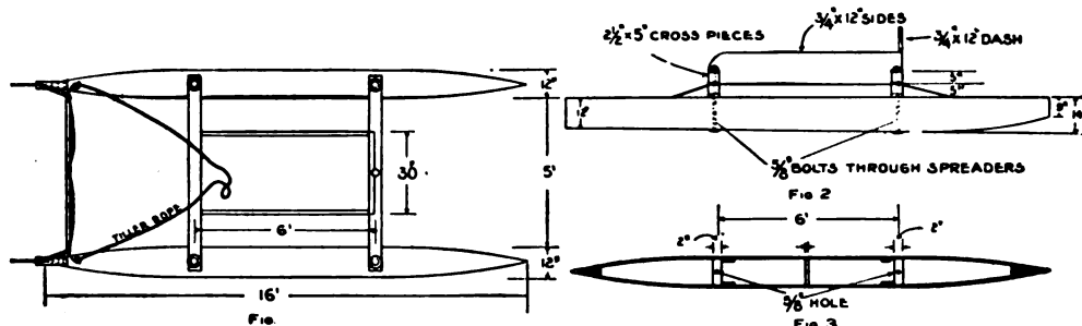
Details of the Pontoons
