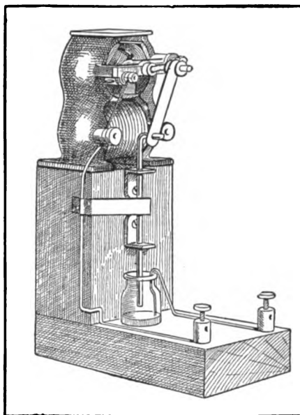
Motor-Driven Make-and-Break
