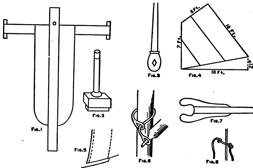
Details of Ice Boat Construction
