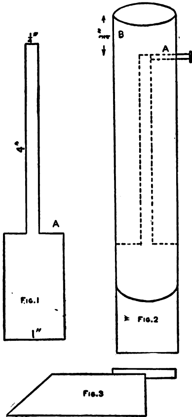
Lead Cannon Construction
