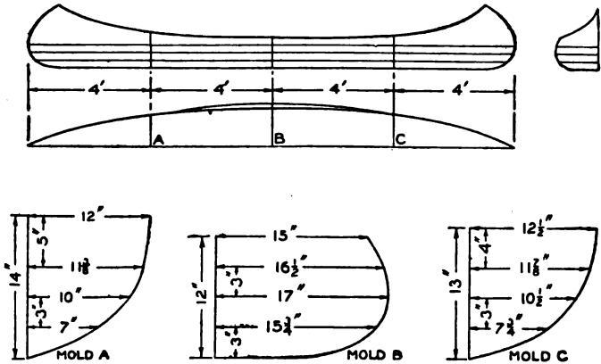
Fig. 1 Canoe and Molds Details
