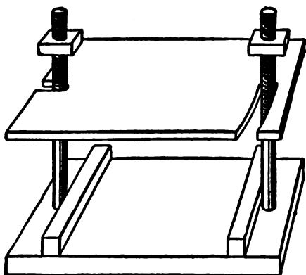
Vulcanizing Press for Rubber Stamps
