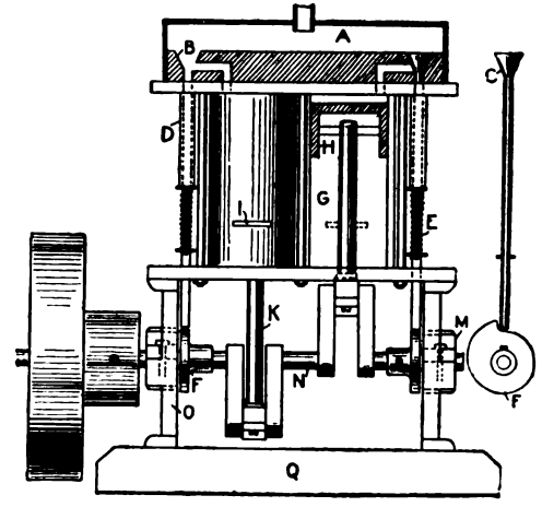
Engine Details
