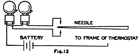
Fig. 12 Wiring Diagram for One and Two Bells
