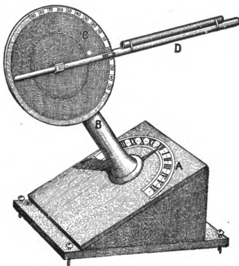
Home-Made Equatorial
