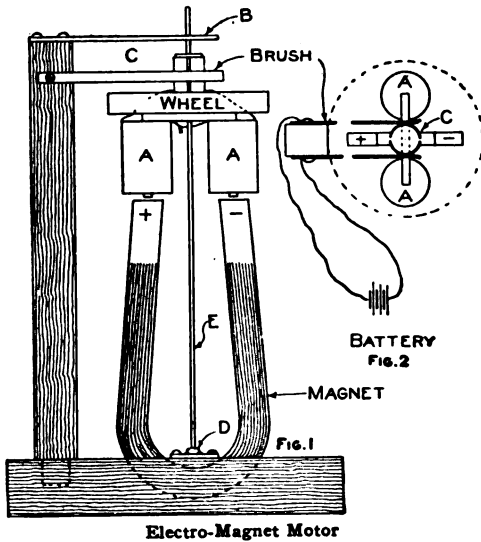
Electro-Magnet Motor
