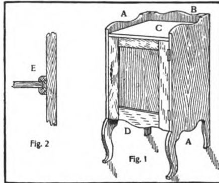
How to Make a Music Cabinet
