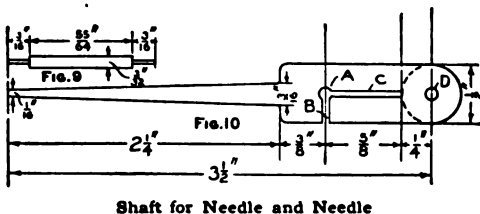
Shaft for Needle and Needle
