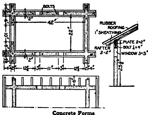
Concrete Forms
