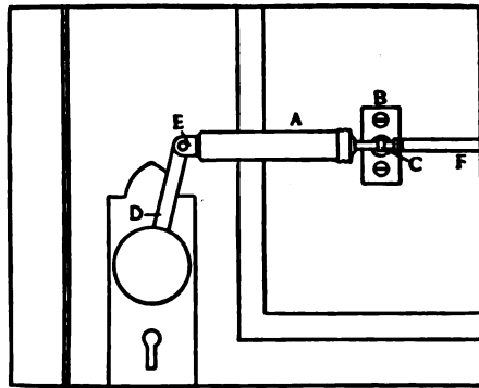
Pneumatic Door-Opener
