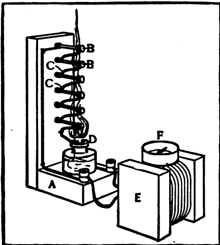
Thermo Battery
