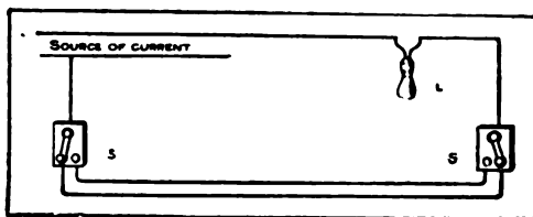
The Wiring Diagram
