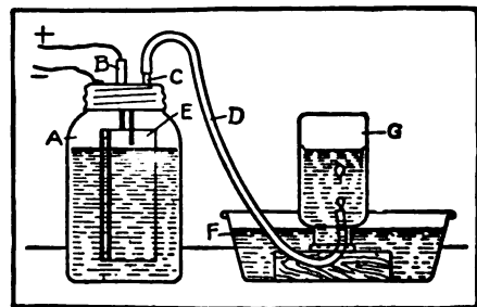
Hydrogen Generator
