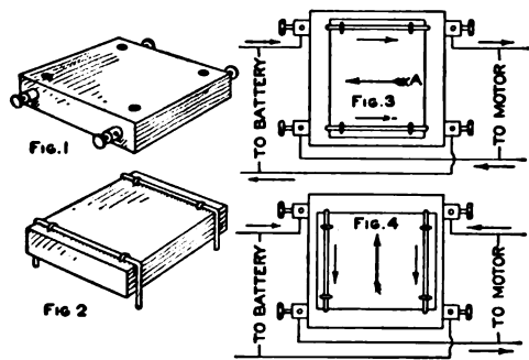
Details of Reverser
