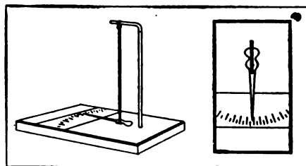
Simple Hygrometer
