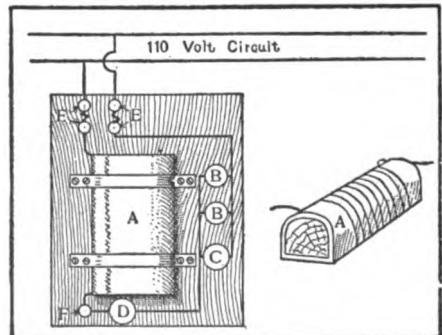
Electric Furnace
